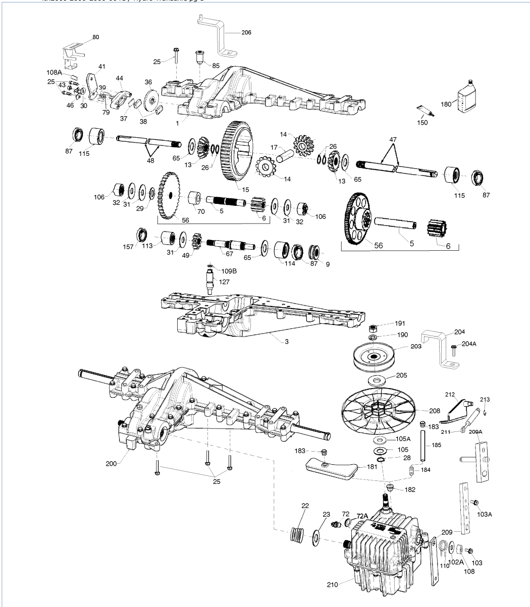
lth2000 2000-2000-004C / Hydro Transaxle pg 1
